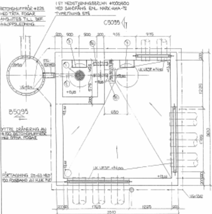
PLAN A 5095 - 120
